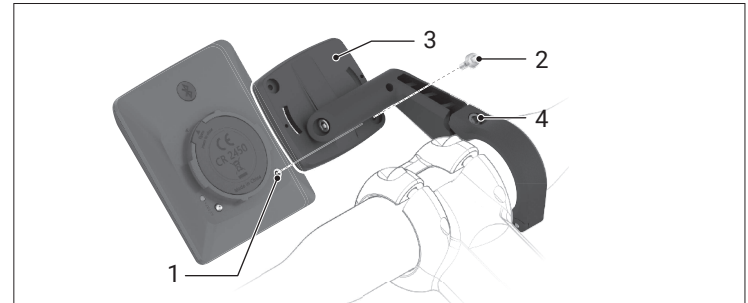
Fig.: 29 Inserting the locking screw
